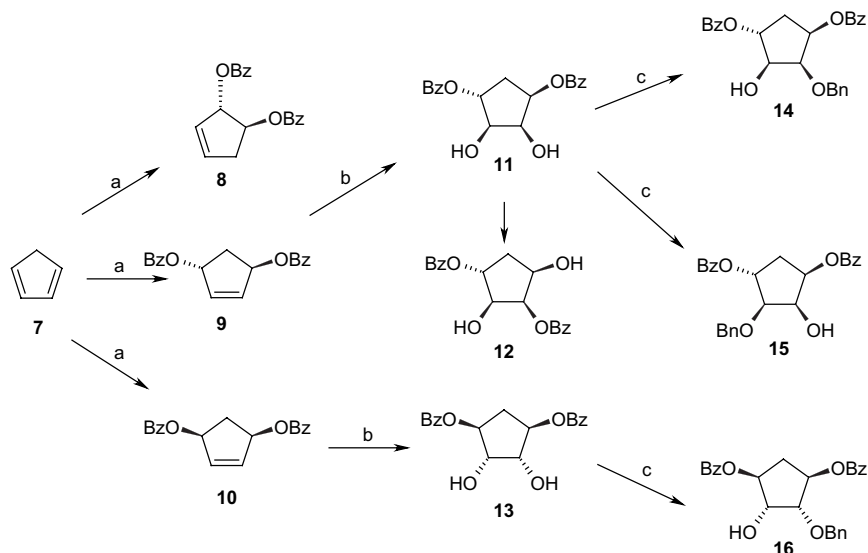
Scheme 1. Reagents and conditions: (a) BzOAg, I 2 , dry Et 2 O, reflux, yield 8–10 63%; (b) KMnO 4 , Me 2 CO, H 2 O, 0 °C, yield 11 33%, 12 17%, 13 66%; (c) Bu 2 SnO, Bu 4 NBr, CH 3 CN, MS 3 Å, BnBr, reflux, yield 14 27%, 15 27%, 16 67%.
