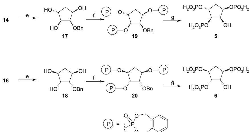
Scheme 2. Reagents and conditions: (e) NaOH 1 N, MeOH, THF, rt, yield 17 41%, 18 85%; (f) N,N -diethylamino benzodioxaphosphorane, 1 H -tetrazole, dry THF, –78 °C, then rt overnight; then –78 °C, m -CPBA, CH 2 Cl 2 , then rt, yield 19 60%, 20 55%; (g) H 2 , 5 atm, Pd/C 10%, MeOH, CH 2 Cl 2 , H 2 O, AcOH, rt, overnight, then evaporation, H 2 O, cyclohexylamine, (Me 2 CO), yield 5 45%, 6 57%.
