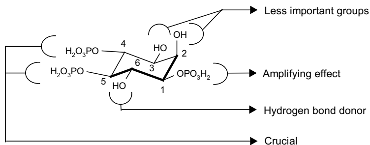
Figure 1. Ins(1,4,5)P 3 pharmacophore model proposed by Kozikowski.
